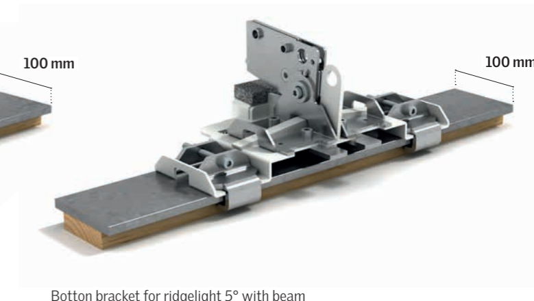
Bottom bracket for ridgetlight 5° with beam
