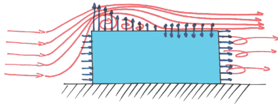
Figur 1: Wind deviation by building (side view)
