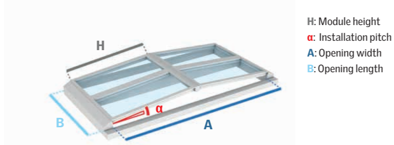
Sub-construction for ridglight at 5° with beam at velux.co.uk/modularskylights
